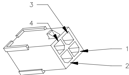
J1 PIN DESIGNATION (2:1 SCALED VIEW)
